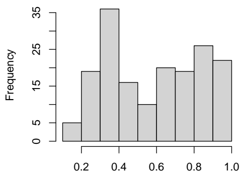
Histogram of PIT values
