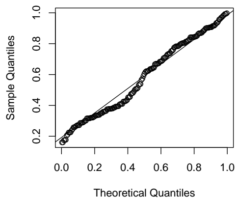
Q-Q plot for Unif(0,1)
